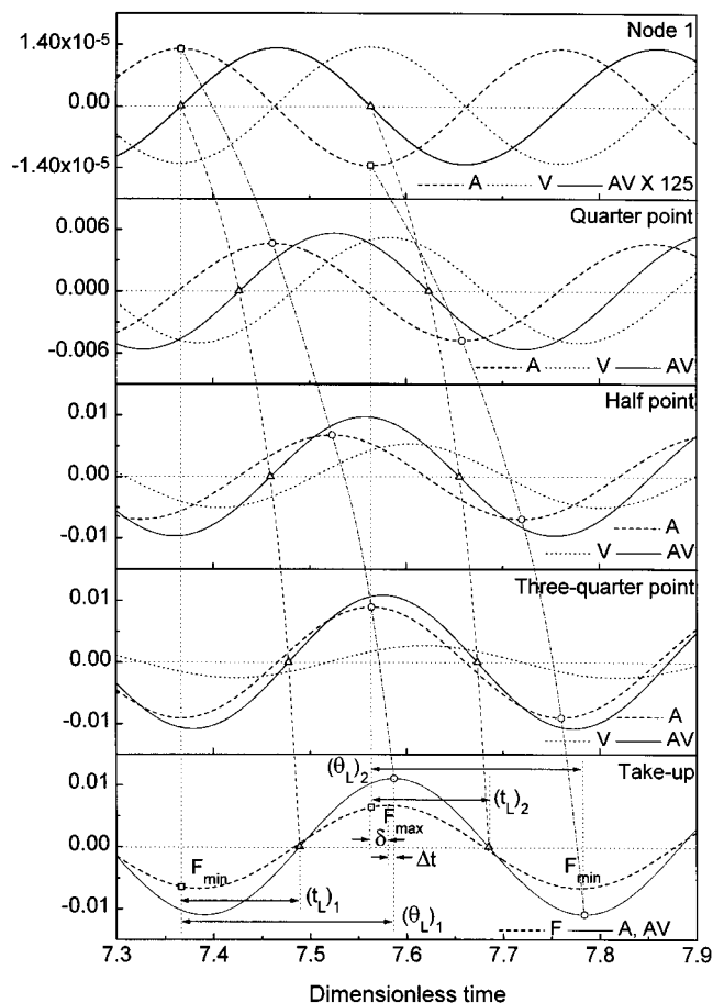
Figure 1. Transient curves of spinline variables at five different spatial points of the spinline when r = r_c = 27.97 for the case of \bar{a} = 0.4 , De = 0.019 .
