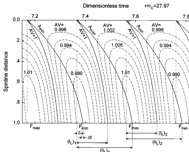
Figure 4. Contours of constant- AV curves when r = r_c = 27.97 for the case of \bar{a} = 0.4 , De = 0.019 .
