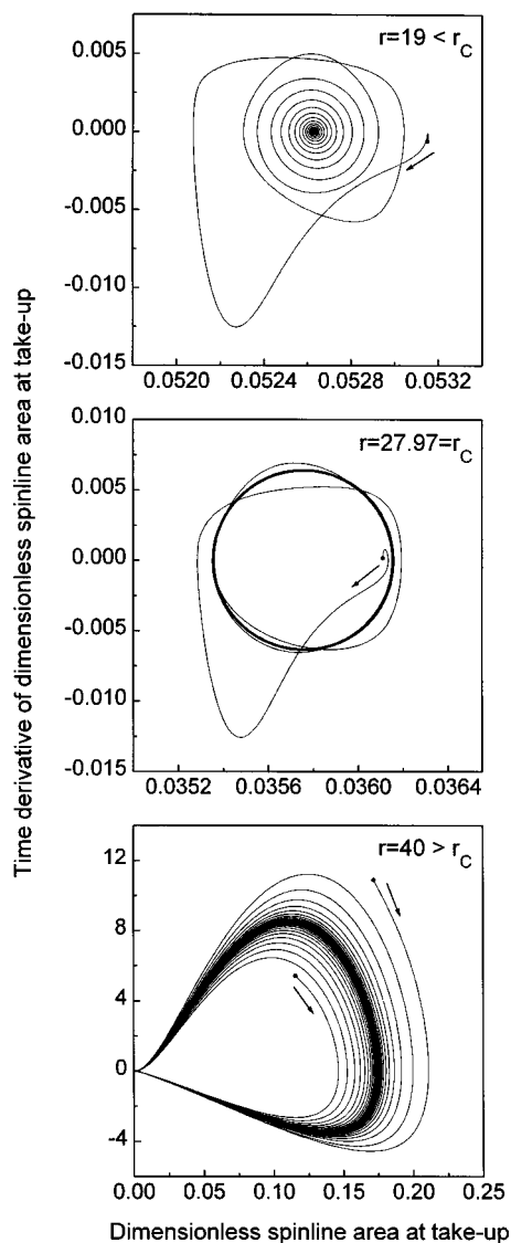
Figure 5. Trajectories of the spinline area at takeup in the phase plane.
