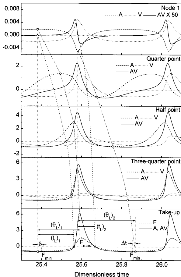
Figure 2. Transient curves of spinline variables at five different spatial points of the spinline when r = 40 > r_c for the case of \bar{a} = 0.4 , De = 0.019 .
